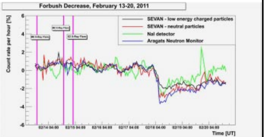
Figure 1: Pressure corrected time series of ASEC particle monitors. This figure shows the intensity variation of the neutral and charged particles measured on Mt. Aragats at 3200 m above sea level.
