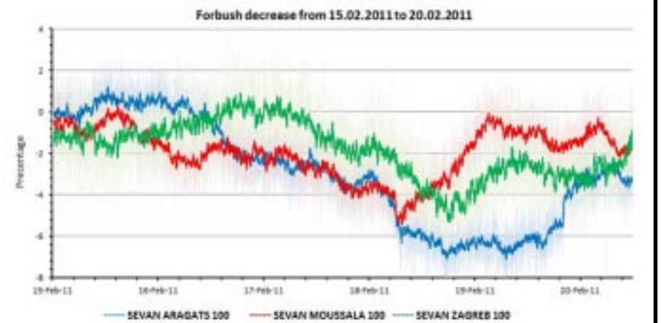
Figure 2: Pressure corrected time series of SEVAN particle monitors. This figure demonstrates the first results from the SEVAN detectors in Armenia, Bulgaria and Croatia, simultaneously registering Fd. The data from monitors located at different longitudes, latitudes and altitudes allows CRD to untangle solar-terrestrial connections and test simulations of fast solar wind interaction with the earth's magnetosphere.
